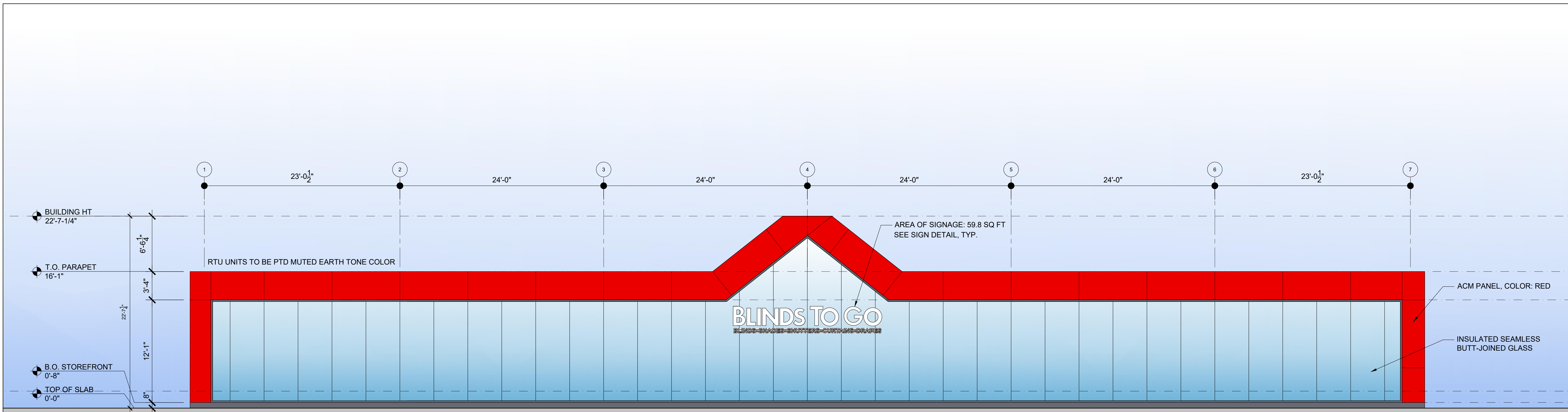
A FRONT ELEVATION (SOUTHWEST) 3/16" = 1'-0" FACADE AREA: 2431.06 SQ. FT.
