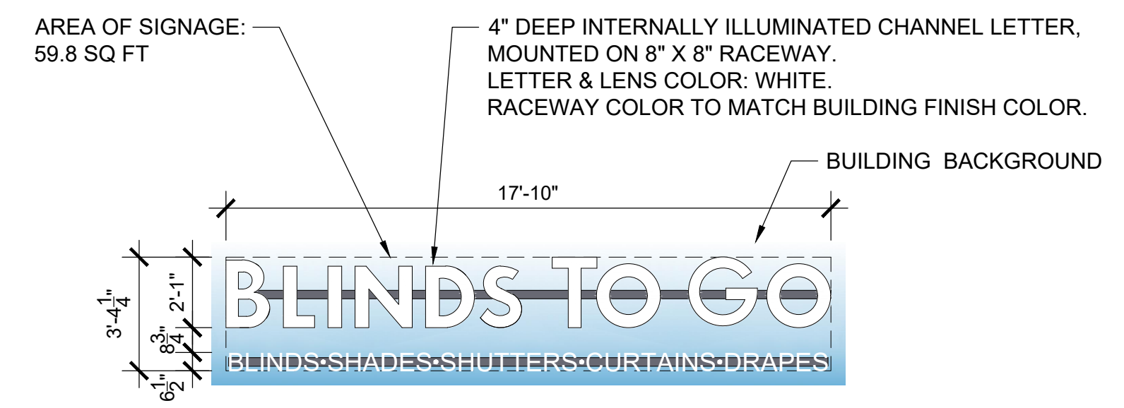
SIGN DETAIL 1/4" = 1'-0"
