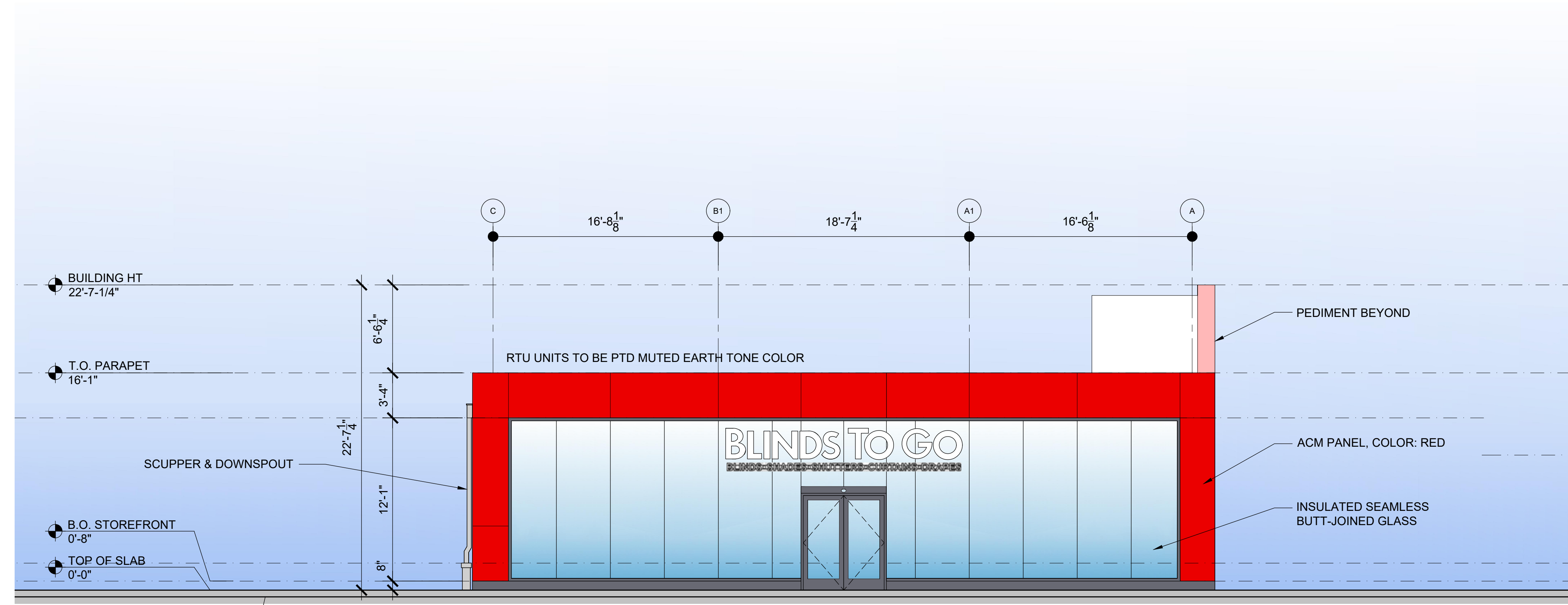
B LEFT SIDE ELEVATION (NORTHWEST) 3/16" = 1'-0" FACADE AREA: 884.58 SQ. FT.
